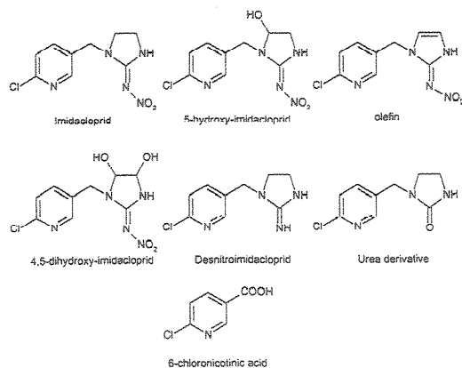
Fig. 1. Structures of imidacloprid and the studied metabolites.
